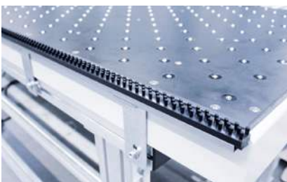
Braking brushes for air cushion table (optional)
