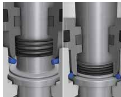
Automatic spindle lock — patented system for a drilling depth that is always accurate for numerous different materials. With speeds from 1500–7500 rpm for high feed speeds or short drill cycles.
